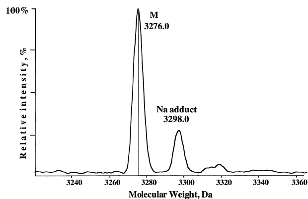
Figure 3. MS analysis (electrospray) of purified chimera V. The sample (PNA–DNA chimera V, 30 µg) was dissolved in 1 ml of 50% water/methanol mixture. One microliter aliquot was taken up and analyzed on a triple quadrupole mass spectrometer API III (PE Sciex, Ontario) equipped with nanoelectrospray ion source developed in EMBL. The figure presents an image deconvoluted using BioMultiview software (PE Sciex, Ontario) from the original spectrum containing the series of multiply charged ions.
