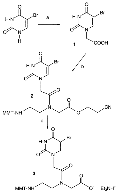
Figure 1. Preparation of the PNA monomer of 5-bromouracil. (a) bromoacetic acid, NaOH; (b) N -(2-(MMT-amino)ethyl)glycine 2-cyanoethyl ester, DIP, HOObt, N -ethylmorpholine; (c) DBU.
