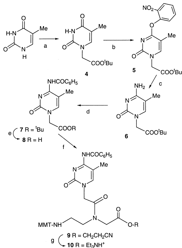
Figure 2. Preparation of the PNA monomer of 5-methylcytosine. (a) t -Butyl bromoacetate, DBU; (b) 2-mesitylenesulfonyl chloride, DMAP followed by o -nitrophenol, 1,4-diazabicyclo[2.2.2]octane; (c) ammonia; (d) benzoyl chloride, pyridine; (e) TFA; (f) N -(2-(MMT-amino)ethyl)glycine 2-cyanoethyl ester, DIP, HOObt, N -ethylmorpholine; (g) DBU.
